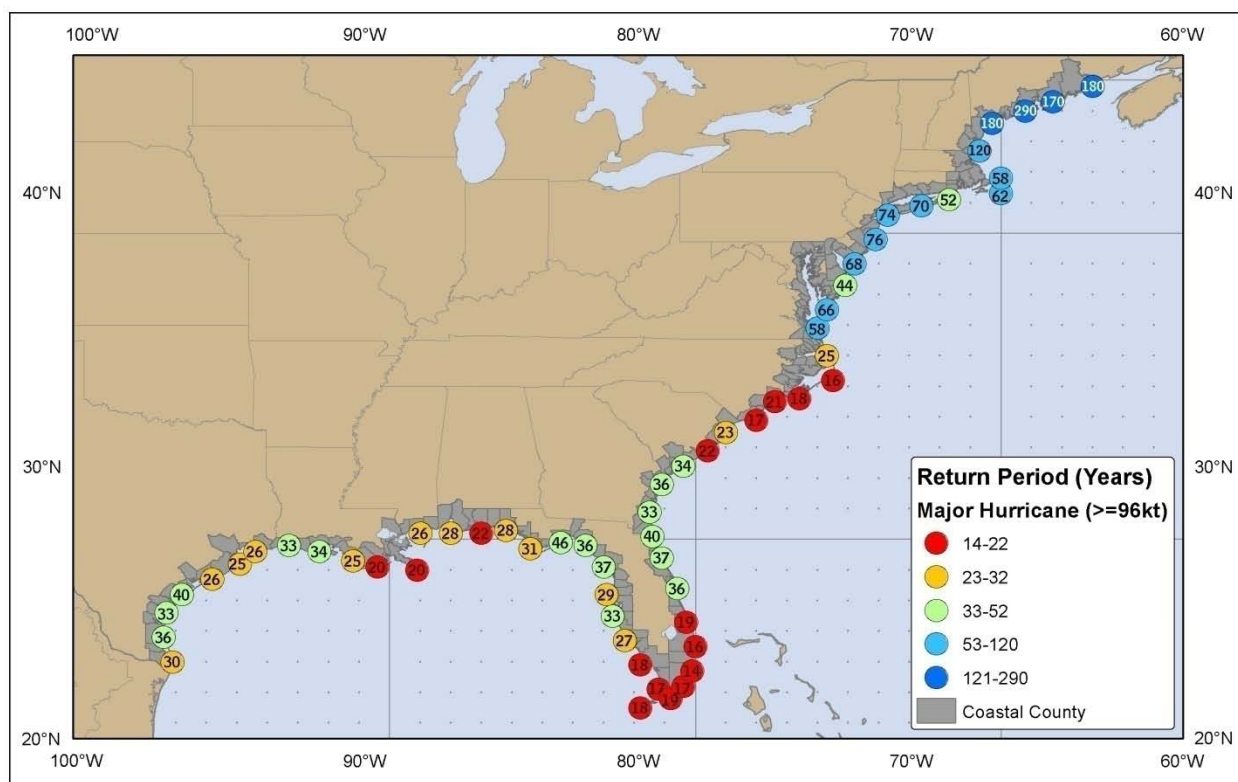
Figure 16: Average Return Periods between Landfalling Major Hurricanes
